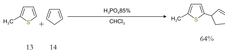
Figure 9. Obtaining 2-(cyclopent-1-en-3-yl)-5-methyl-thiophene
