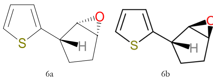
Figure 3. Structures of epimers
