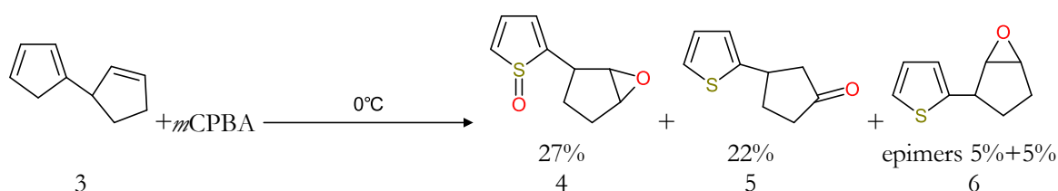
Figure 5. Oxidation of 2-(cyclopent-1-en-3-yl)thiophene from 1.5 mol of methachloroperoxybenzoic acid
