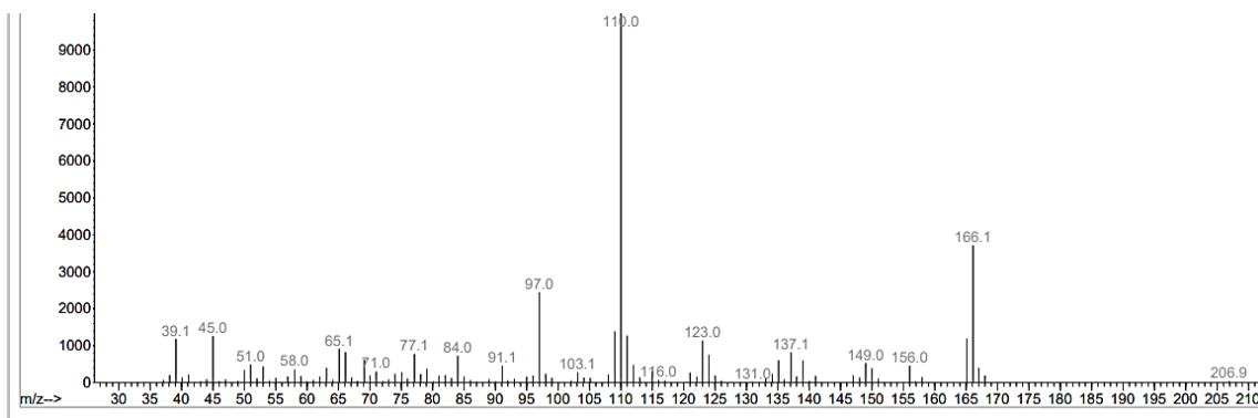
Figure 16. Fragment of the GCMS spectrum of compound (6)
