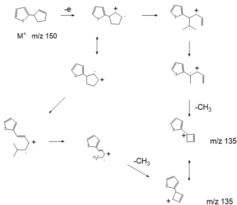
Figure 15. Decomposition of 2-(Cyclopent-1-en-3-yl)thiophene (3)
