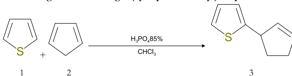
Figure 1. Obtaining 2-(cyclopent-1-en-3-yl)thiophene
