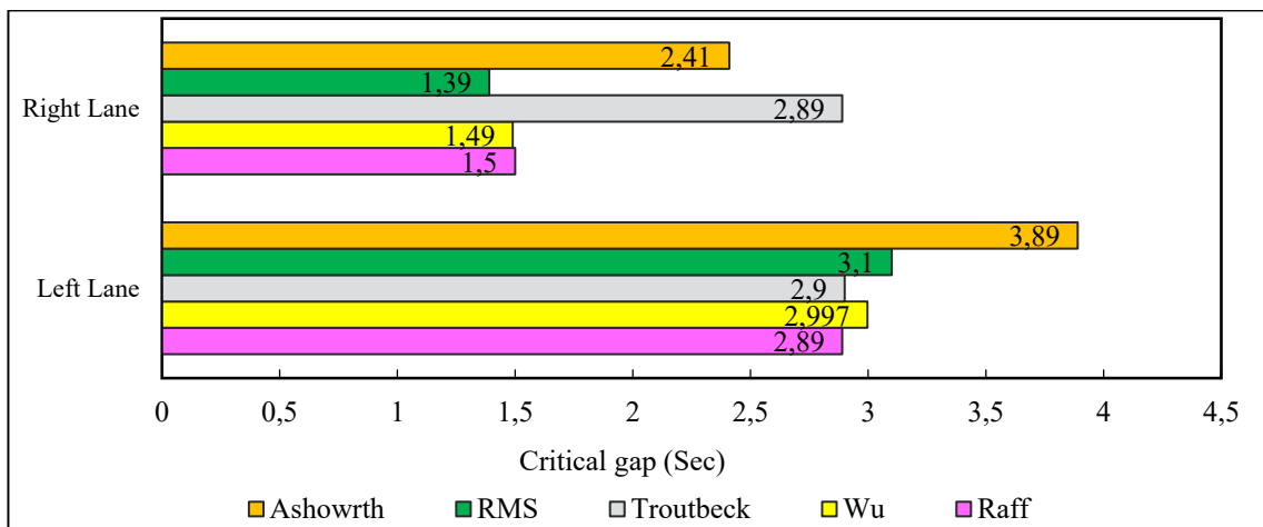
Figure 5. Results for each method of estimating the critical interval
